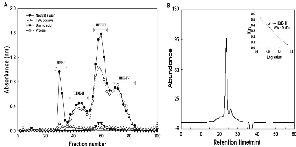
Fig. 1. Elution profiles of crude polysaccharides (HBE-0) isolated from the pectinase digests of Citrus Hallabong peel on the column of Sephadex G-75 by GPC (gel permeation chromatography). ●, Neutral sugar (490 nm); ○, TBA positive material (548 nm); ▼, Uronic acid (520 nm); ▽, Protein (600 nm).
